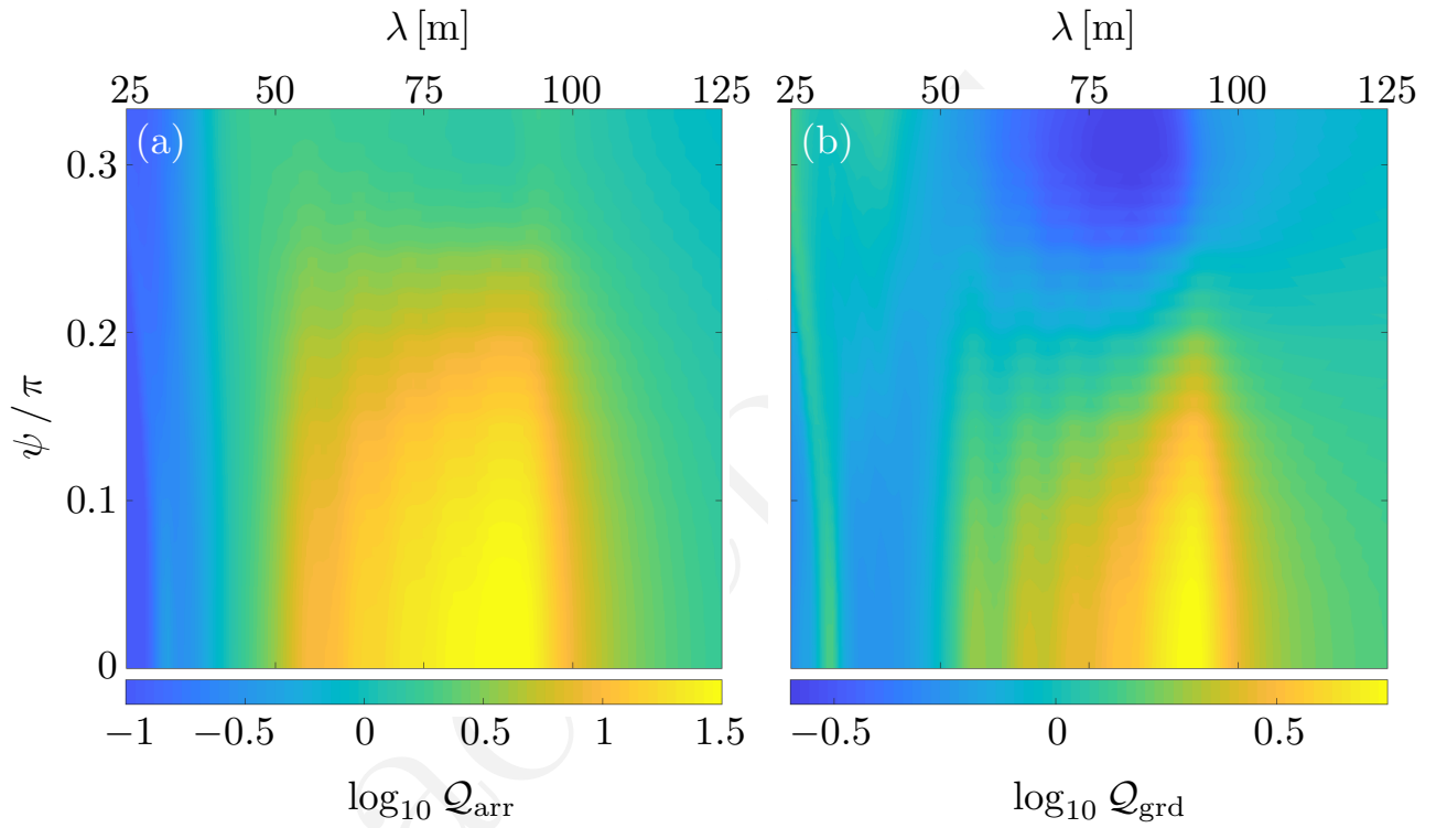
Figure 4: Logarithmic Q-factors as functions of incident wavelength and direction. (a) Q_{\text{arr}} = \mathcal{E} / \mathcal{E}_{\text{inc}} , where \mathcal{E} is the integrated energy within the C-shaped cylinders along the array, and \mathcal{E}_{\text{inc}} is the incident energy over the same domain. (b) Q_{\text{grd}} = \mathcal{E} / \mathcal{E}_0 , where \mathcal{E}_0 is the integrated energy within equivalent isolated C-shaped cylinders.
